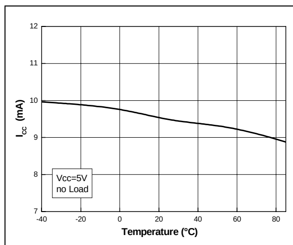
Figure 18. Supply current vs. temperature
